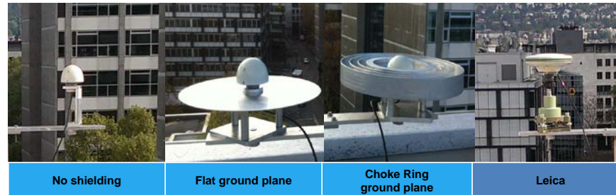
Four combinations of antenna-shieldings
