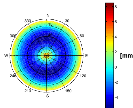
PCV of TBIII antenna with flat Ground Plane and Choke Ring Ground Plane
