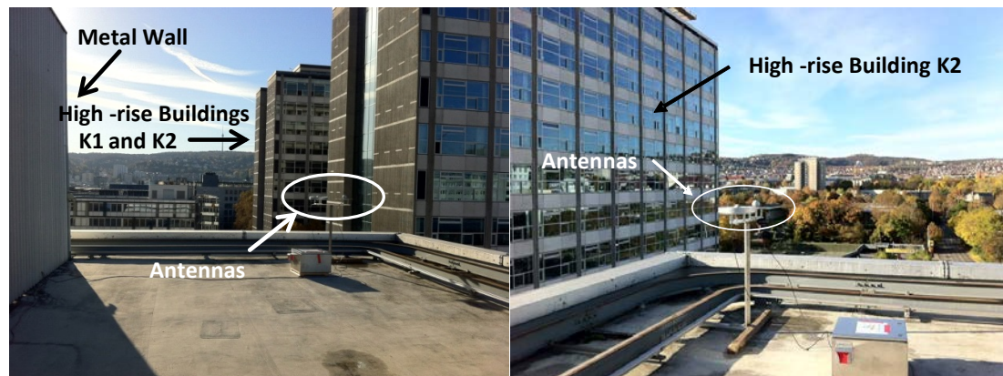
Photos of Test Field
