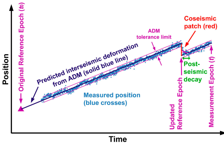
Figure 7: Observed and modeled deformation through time.
