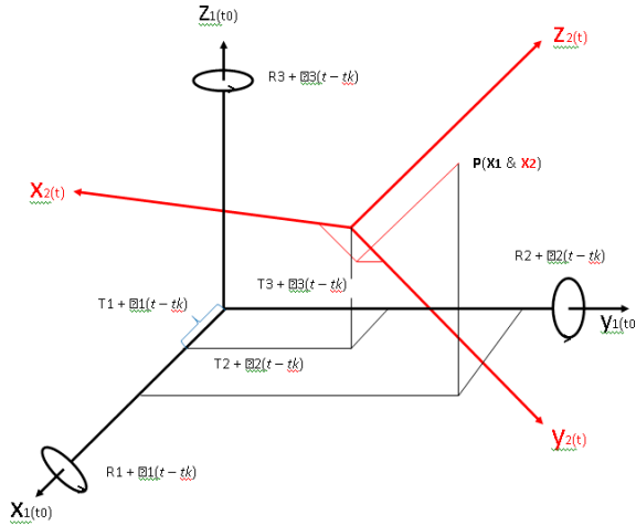
Figure 6: Diagram showing the parameters of a general transformation between two 3-D coordinate systems.
