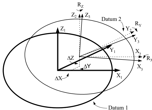
Figure 9: Diagram showing the 7-parameters of transformation between two ellipsoids.
