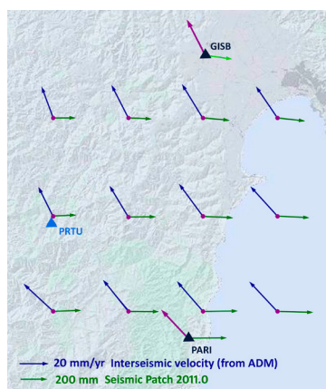
Figure 8: Interseismic velocities and seismic patch deformation.
