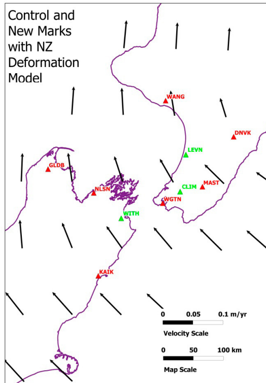
Figure 10: Existing stations (red triangles), new stations (green triangles) and gridded velocities.
