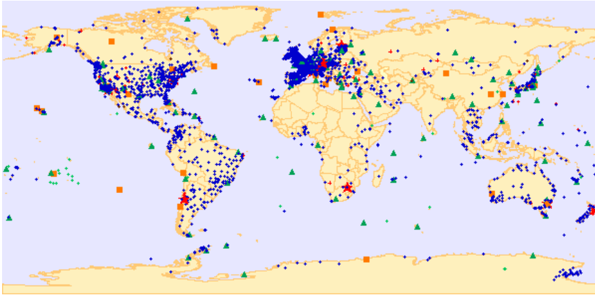
Figure 4: Geodetic reference stations.
